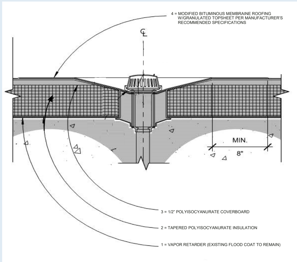
New Roof Cross Section
